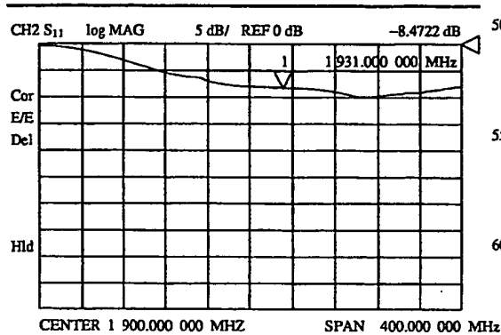
Return loss characteristic of the antenna in free space.
